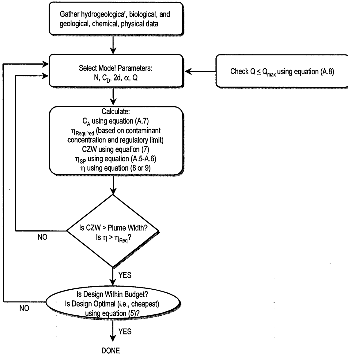
Figure 5-1. Flow Diagram for System Design
